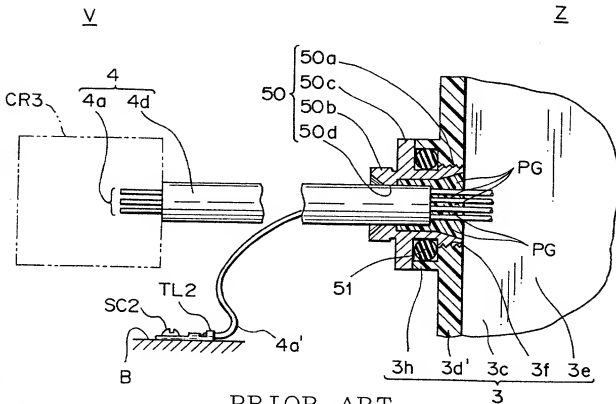
PRIOR ART FIG. 13
